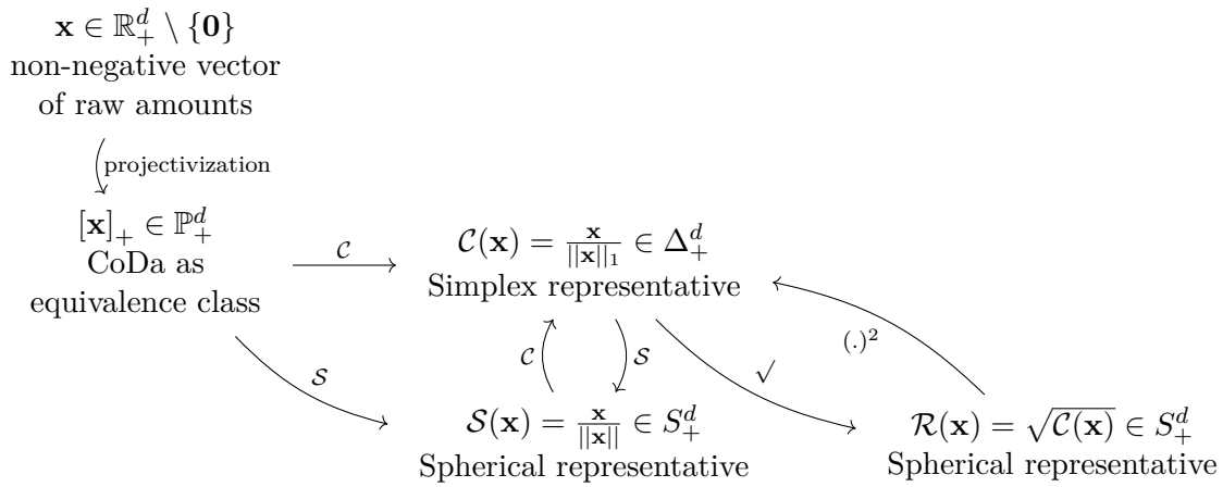
Figure 1: Normalized spherical representations \mathcal{S}(\mathbf{x}) or \mathcal{R}(\mathbf{x}) on the non-negative unit Euclidean sphere S_+^d of a CoDa [\mathbf{x}]_+
